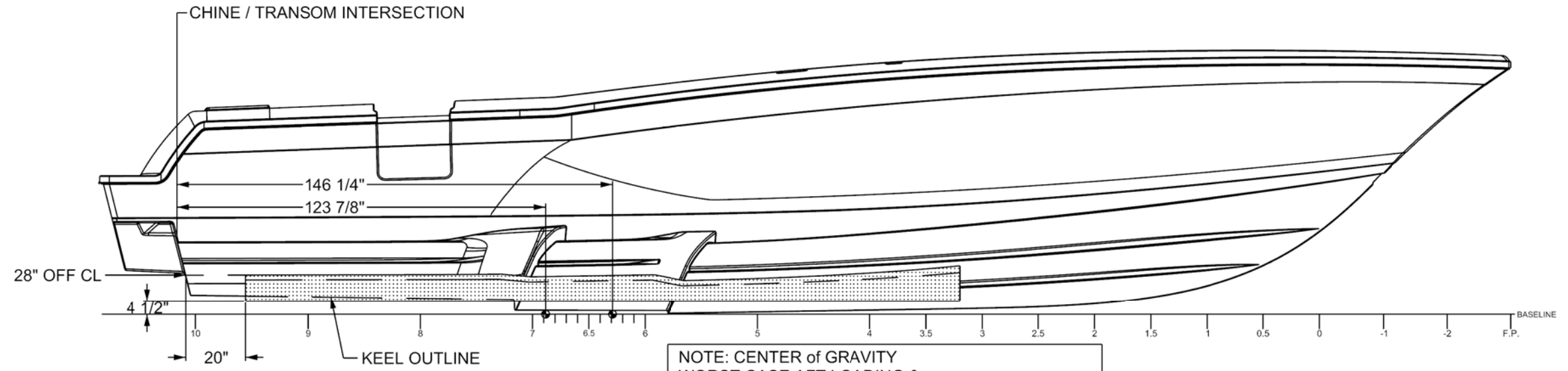
PROFILE SCALE: 3/4" = 1'-0"
