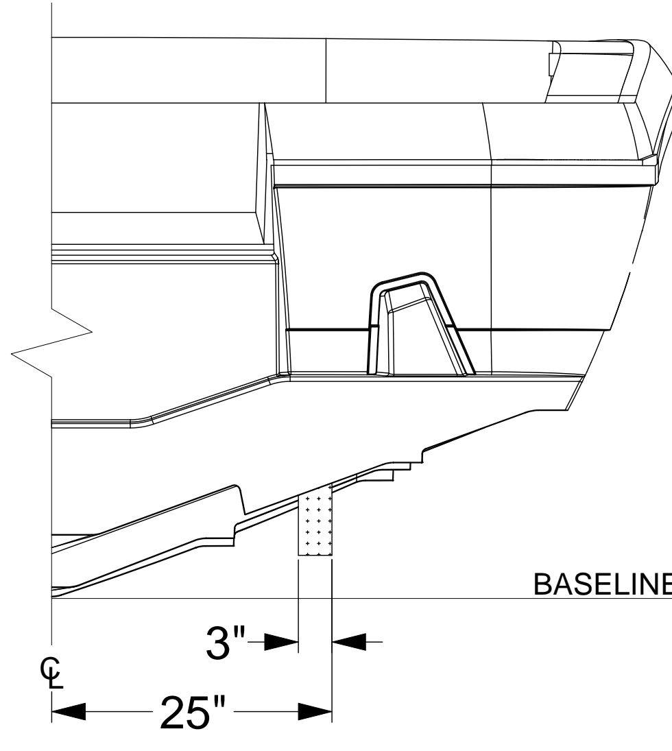
STERN ELEVATION SCALE: NOTED
