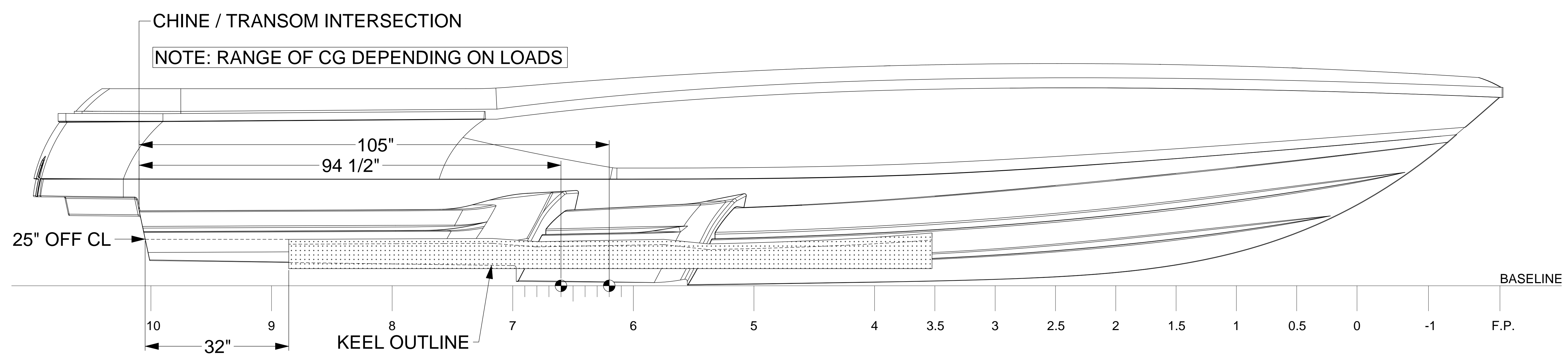
PROFILE SCALE: NOTED
